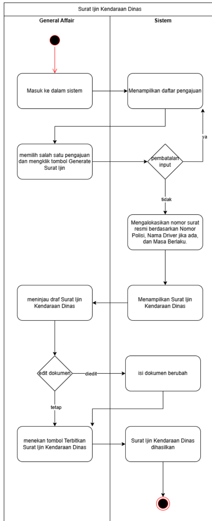
Gambar 3. 26 Activity Diagram Surat Ijin Kendaraan Dinas
